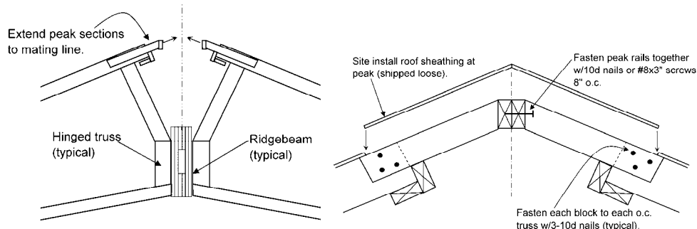
Figure 24. Ridge Assembly
