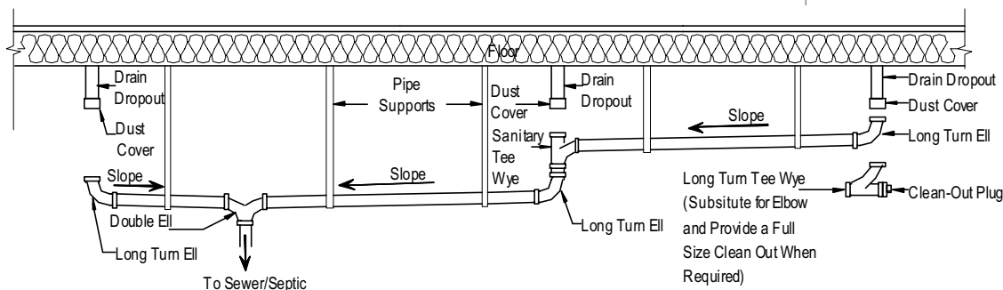
Figure 64. DWV system
