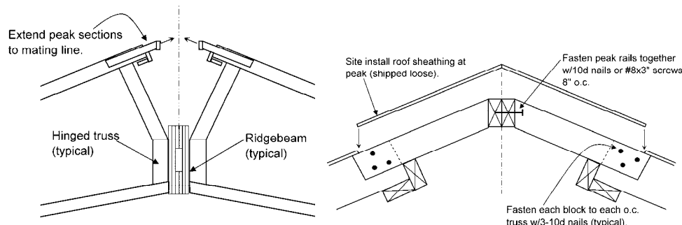
Figure 24. Ridge Assembly
