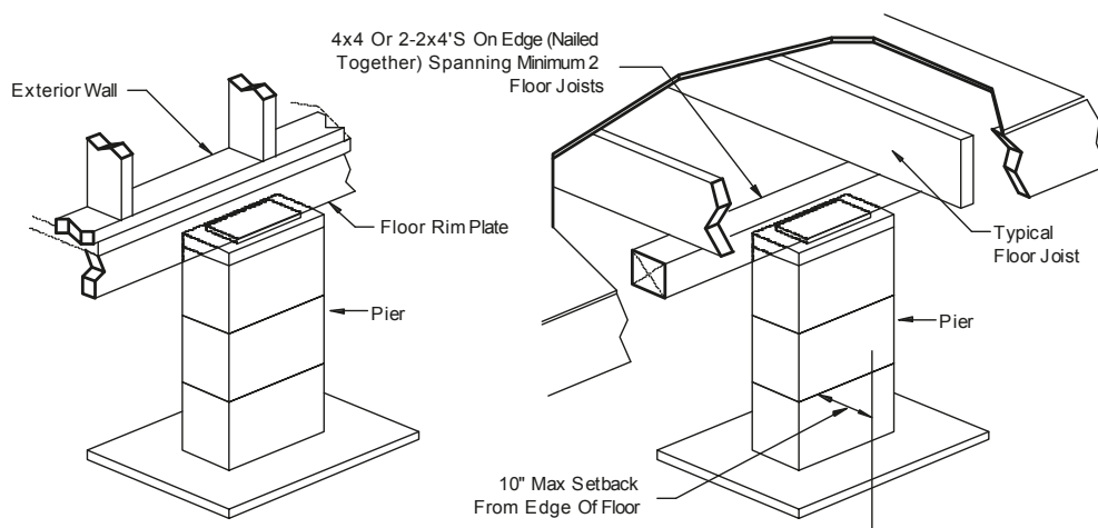
Figure 14. Perimeter supports
