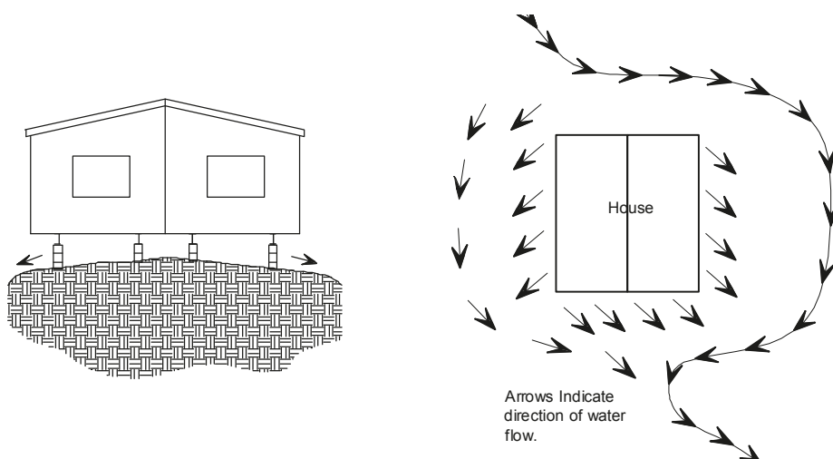
Figure 4. (Left) Crown the soil under the home to prevent water ponding
