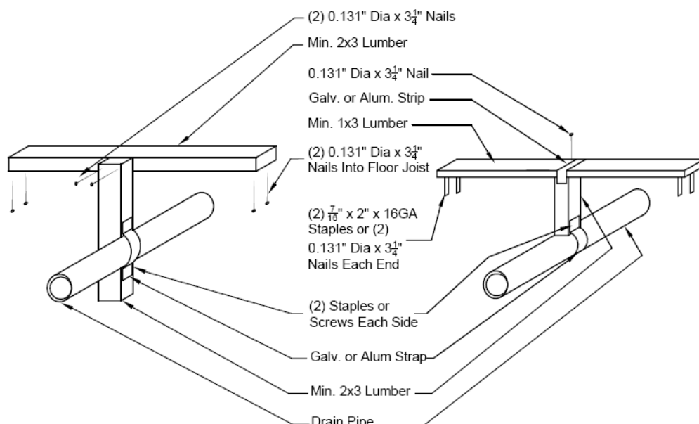
Figure 66. DWV pipe optional support method
