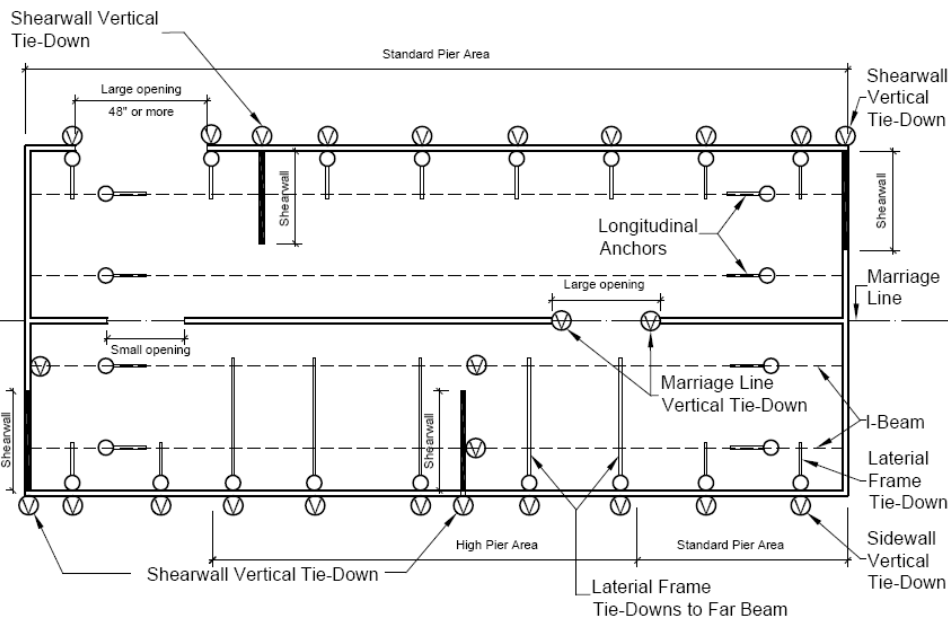
Figure 70. Typical anchor locations for a double-section home in Wind Zones II or III
