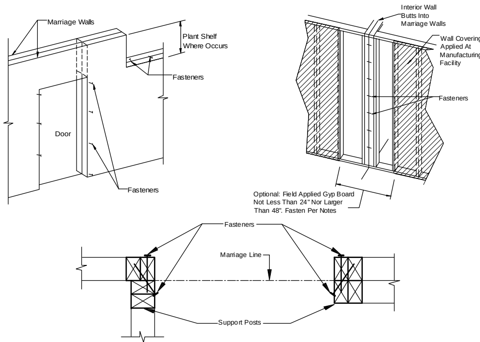
Figure 41. Marriage wall connections
