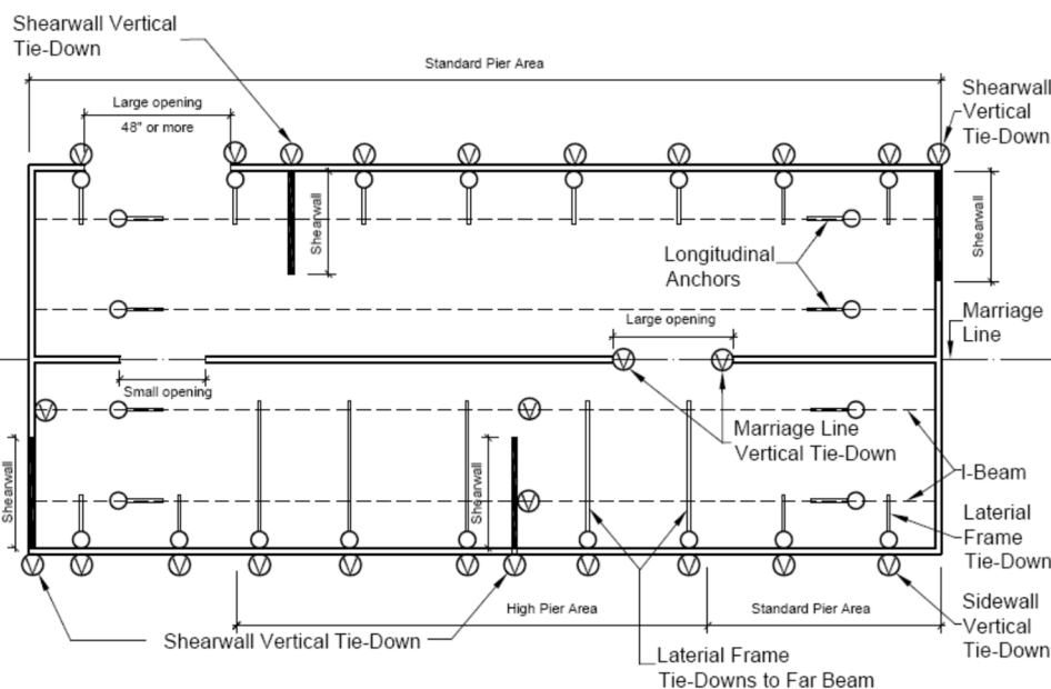
Figure 70. Typical anchor locations for a double-section home in Wind Zones II or III
