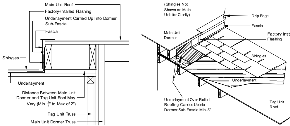
Figure 39. Tag unit roofing connection with less than two inch height difference
