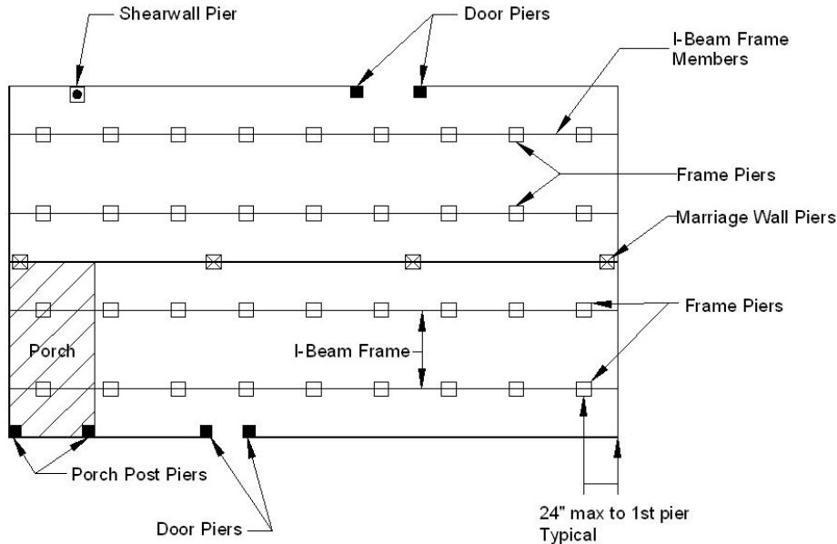
Figure 10. Typical support locations for homes not requiring regularly spaced perimeter supports
