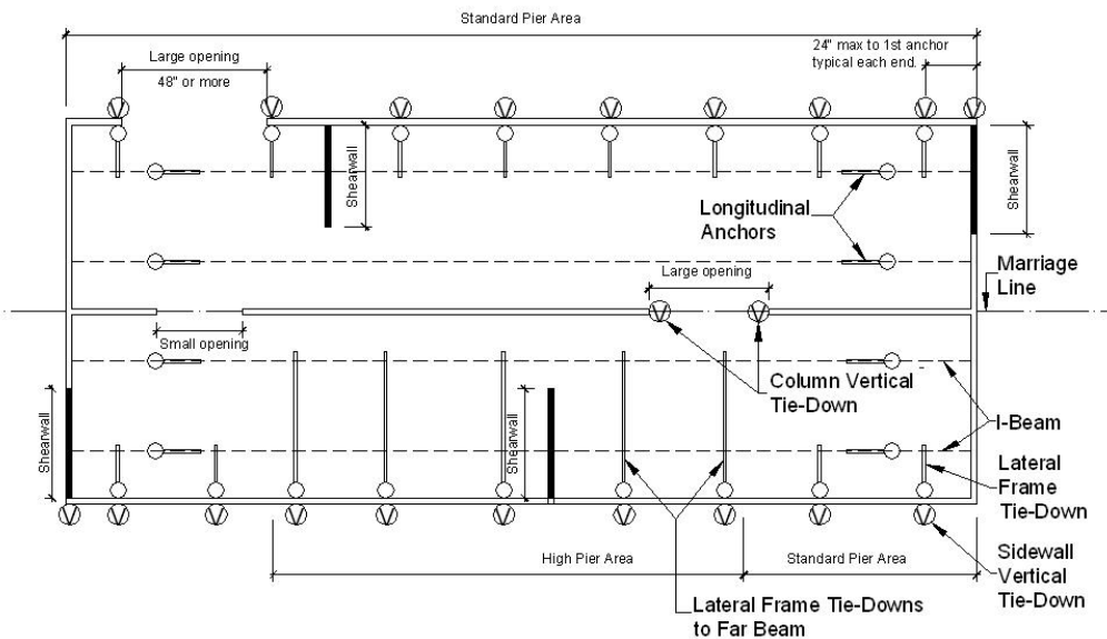
Figure 62. Typical anchor locations for a double-section home in Wind Zones II or III
