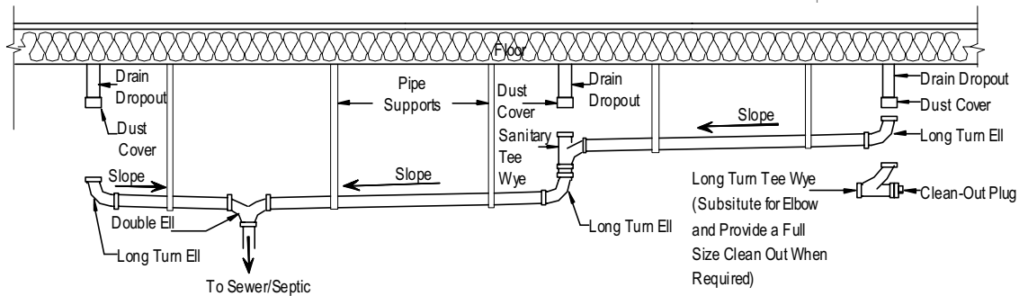
Figure 56. DWV system
