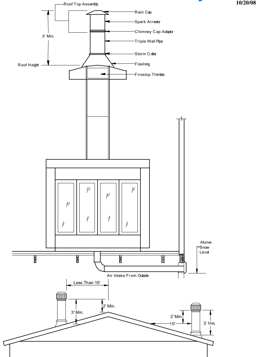
Figure 85. Chimney and combustion air intake duct installation
