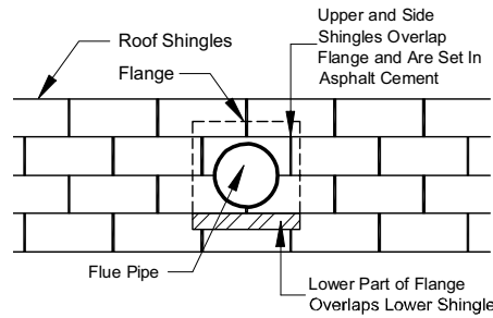
Figure 87. Roof flashing and shingle installation around chimney
