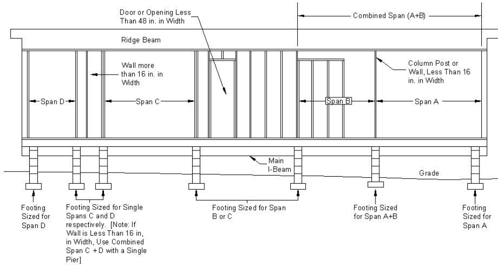
Figure 9. Typical point-load support locations along the marriage line
