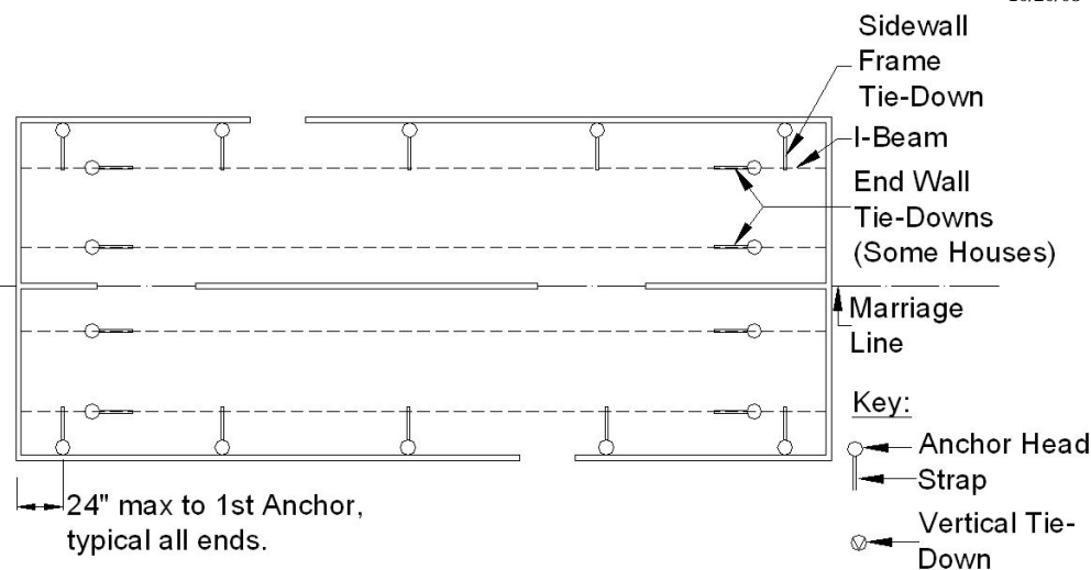
Figure 61. Typical anchor locations for a double-section home in Wind Zone I
